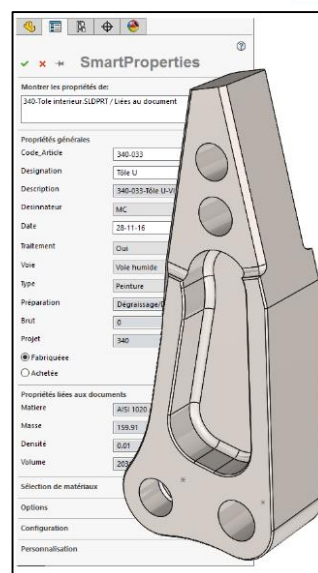
Outil SmartProperties
